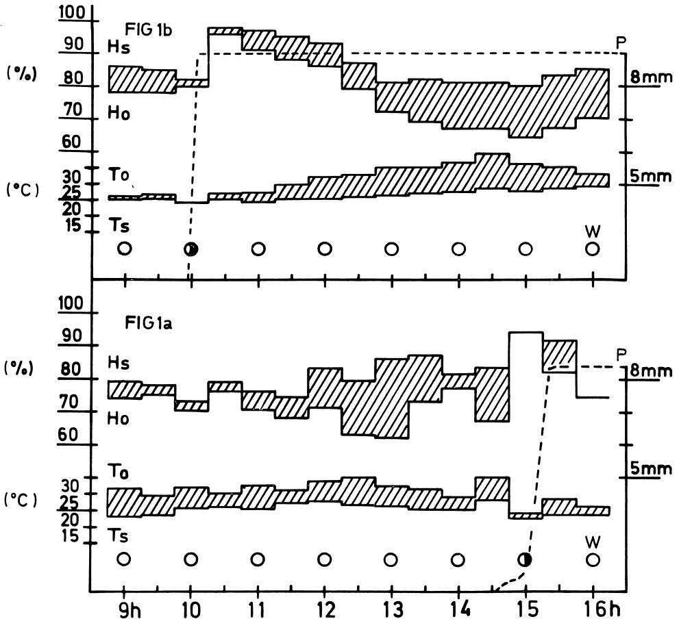
Fig. 1a/1b: "Diurnal march" of maximum air temperature (stand = Ts, open = To), relative air humidity (stand = Hs, open = Ho), precipitation (P) and mean wind velocity (W) at the Acapu (1a—4/10/68) and Andiroba (1b—2/10/68) plot.
