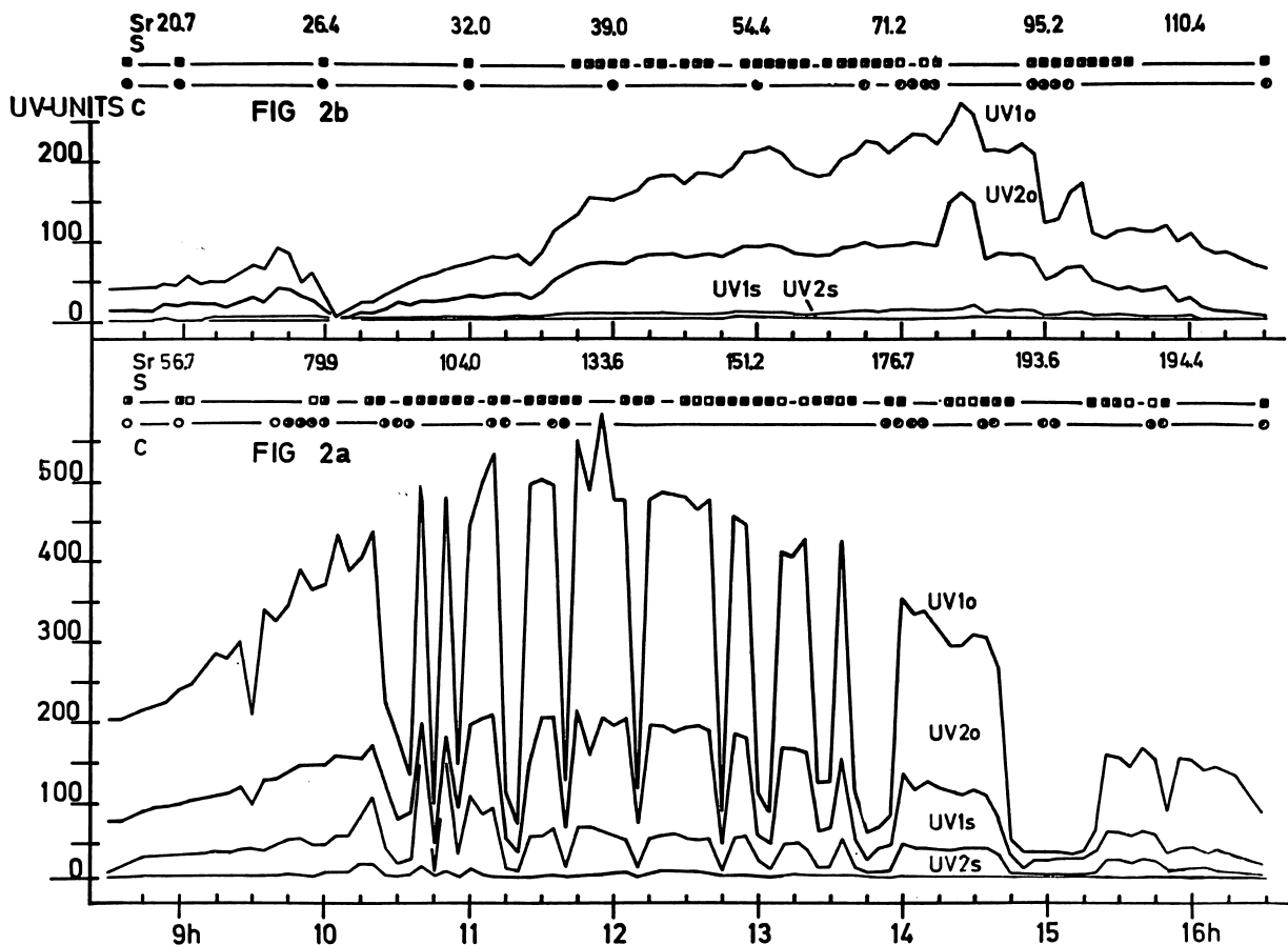
Fig. 2a/2b: "Diurnal march" of UV-1 (open)-, UV-1 (stand)-, UV-2 (open)-, UV-2 (stand)-radiation, solar radiation (Sr), sunshine (S) and cloudiness (C) of the Acapu (2a — 4/10/68) and Andiroba (2b — 2/10/68) plot.
